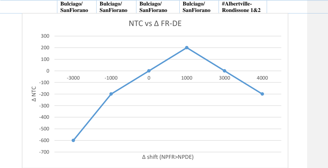
Figure 14: NTC value with Delta shift variation
