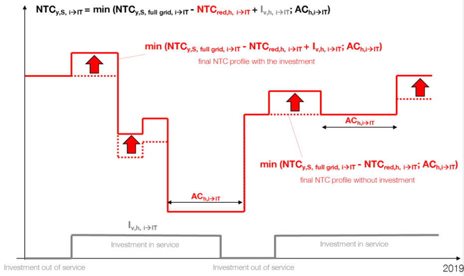
Figure 11 : Final NTC hourly profile computation considering the general inclusion of a new grid investment and its hourly Investment value profile (according its availability plan).
