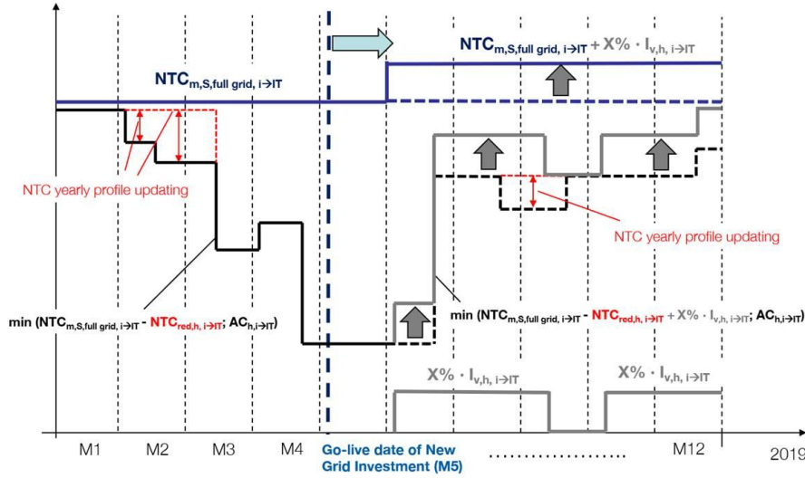
Figure 7: Treatment of Go Live of New Grid Investment(s) for the monthly profile computation
