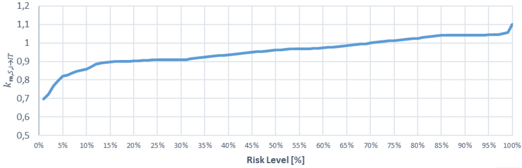
Figure 8 : Duration curve of k_{m,S,i \rightarrow IT} factor
