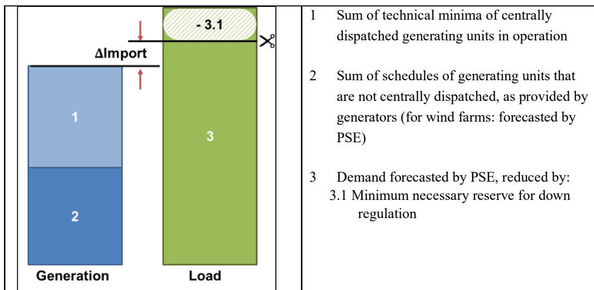
Figure 2: Determination of external constraints in import direction (reserves in generating capacities available for potential imports) in the framework of intraday capacity calculation. Frequency of re-assessment
