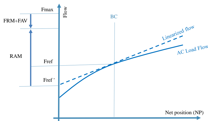
Figure 6-1 Relation between flow, net position and RAM
