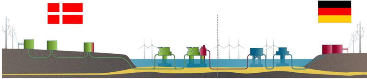
Figure 2 Conceptual sketch of KF CGS that is constituted of parts from a Danish OWF (with two offshore substations), two German OWFs, a connecting cable between the OWFs, and a back-to-back converter station. Green colours indicate parts of KF CGS stemming from the Danish OWF, blue colours show parts stemming from the German OWFs, and red colours show parts stemming from the CCR Hansa interconnector.
