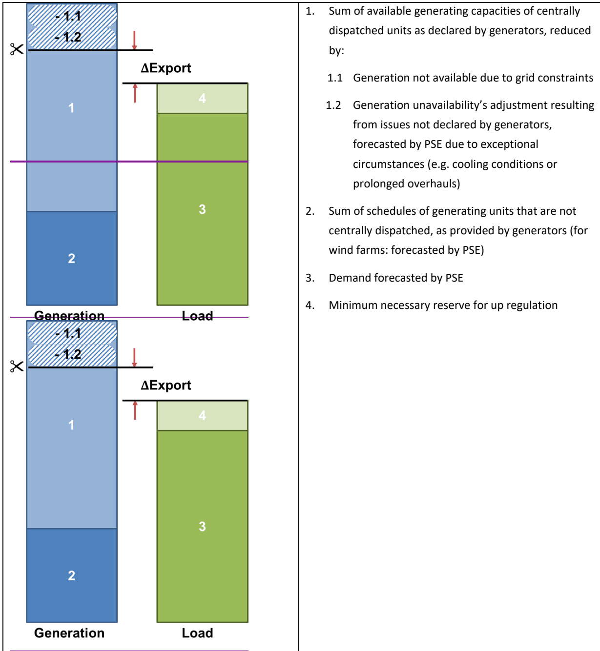
Figure 1: Determination of allocation constraints in export direction (generating capacities available for potential exports) in the framework of day-ahead transfer capacity calculation.
