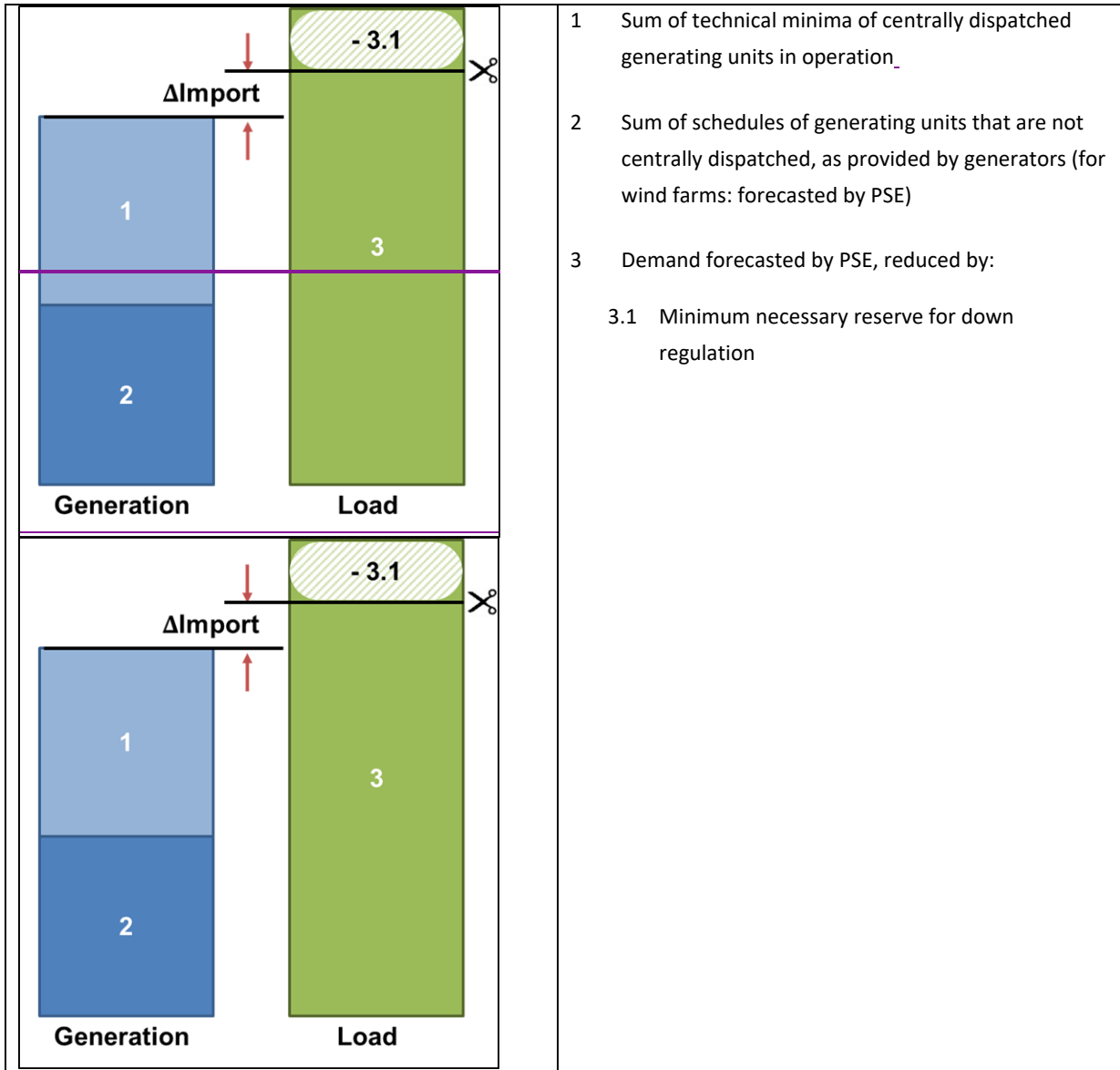
Figure 2: Determination of allocation constraints in import direction (reserves in generating capacities available for potential imports) in the framework of day-ahead transfer capacity calculation.
