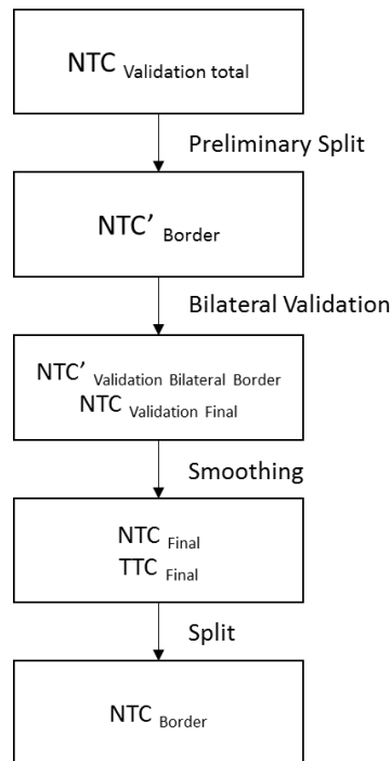
Figure 4: NTC Calculation diagram
